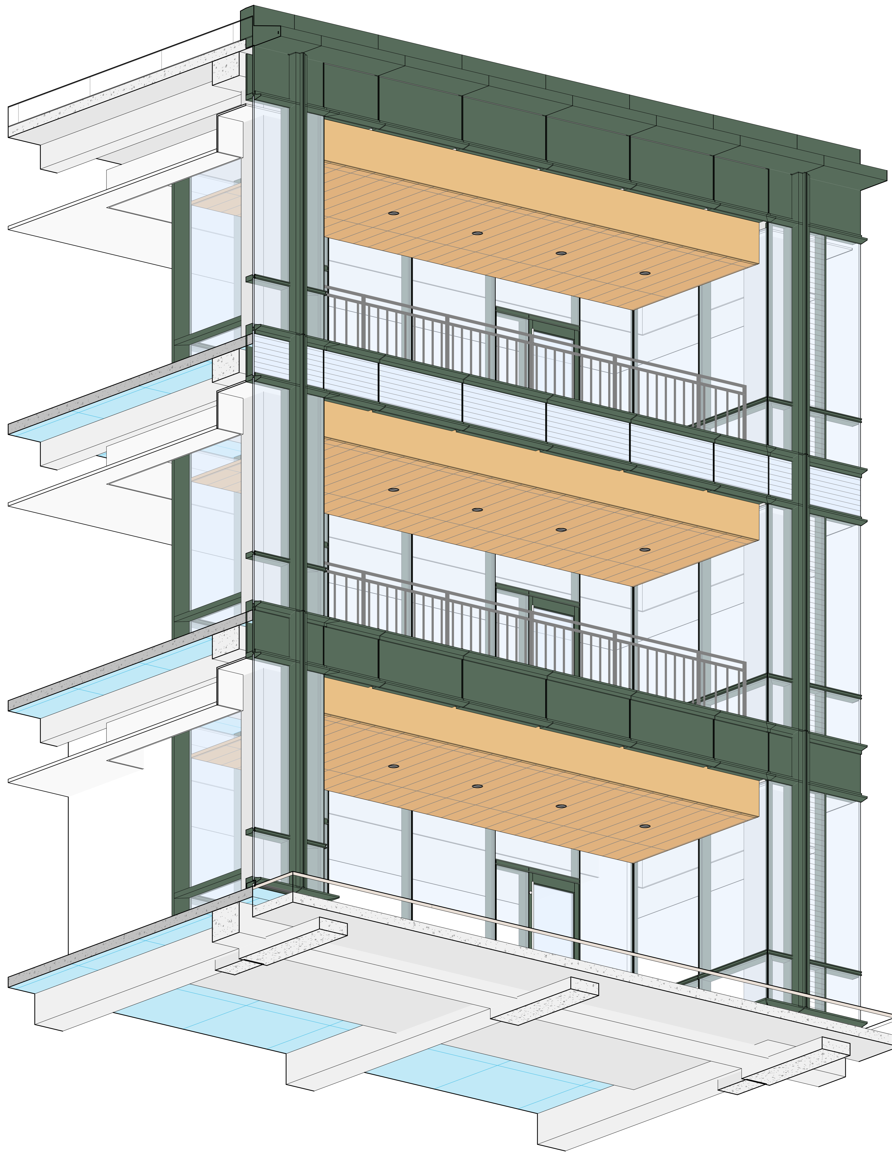
2 ENCLOSURE TYPE A2 - INSET TERRACE CEILING - AXON
