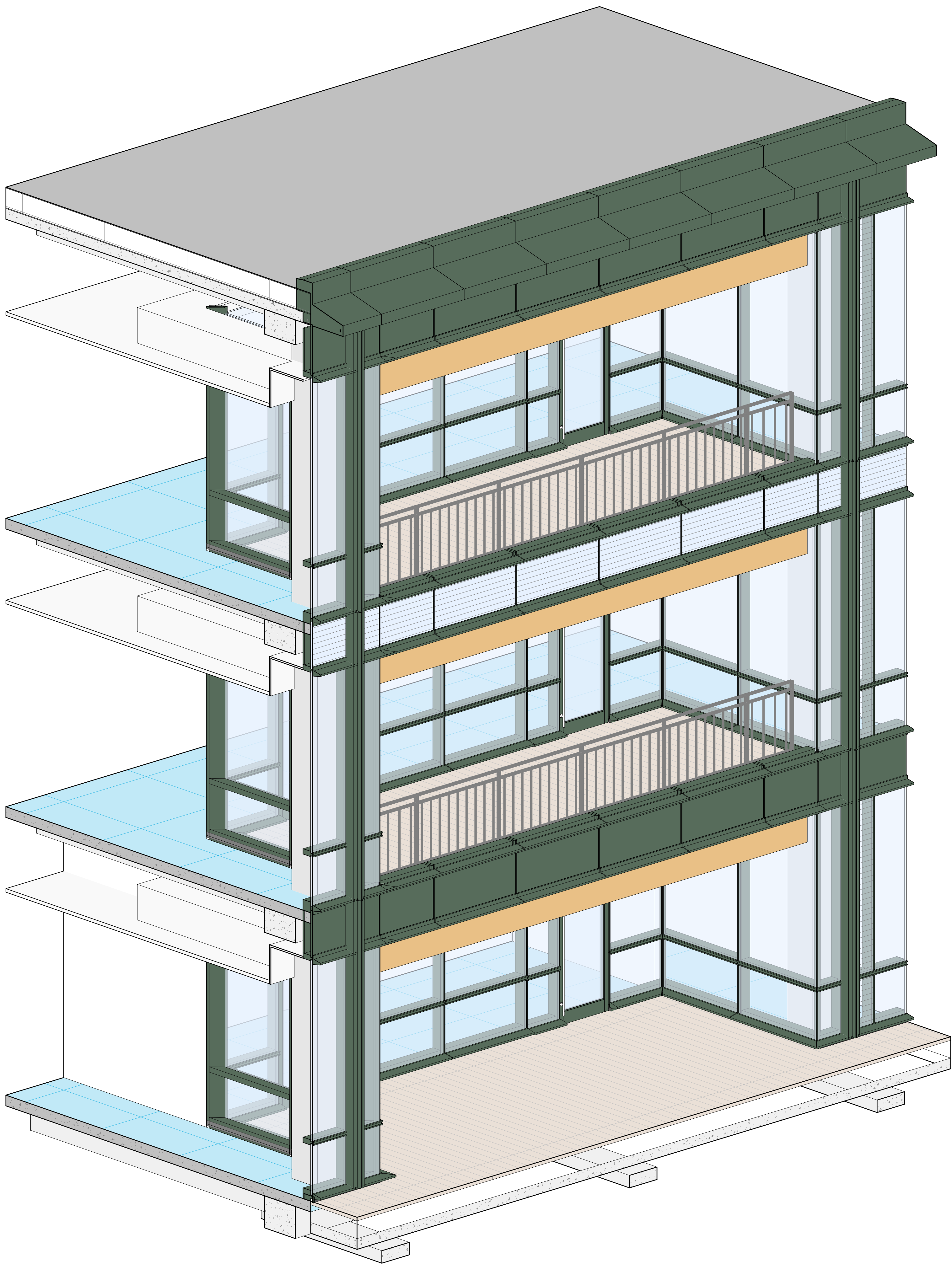
1 ENCLOSURE TYPE A2 - INSET TERRACE - AXON
